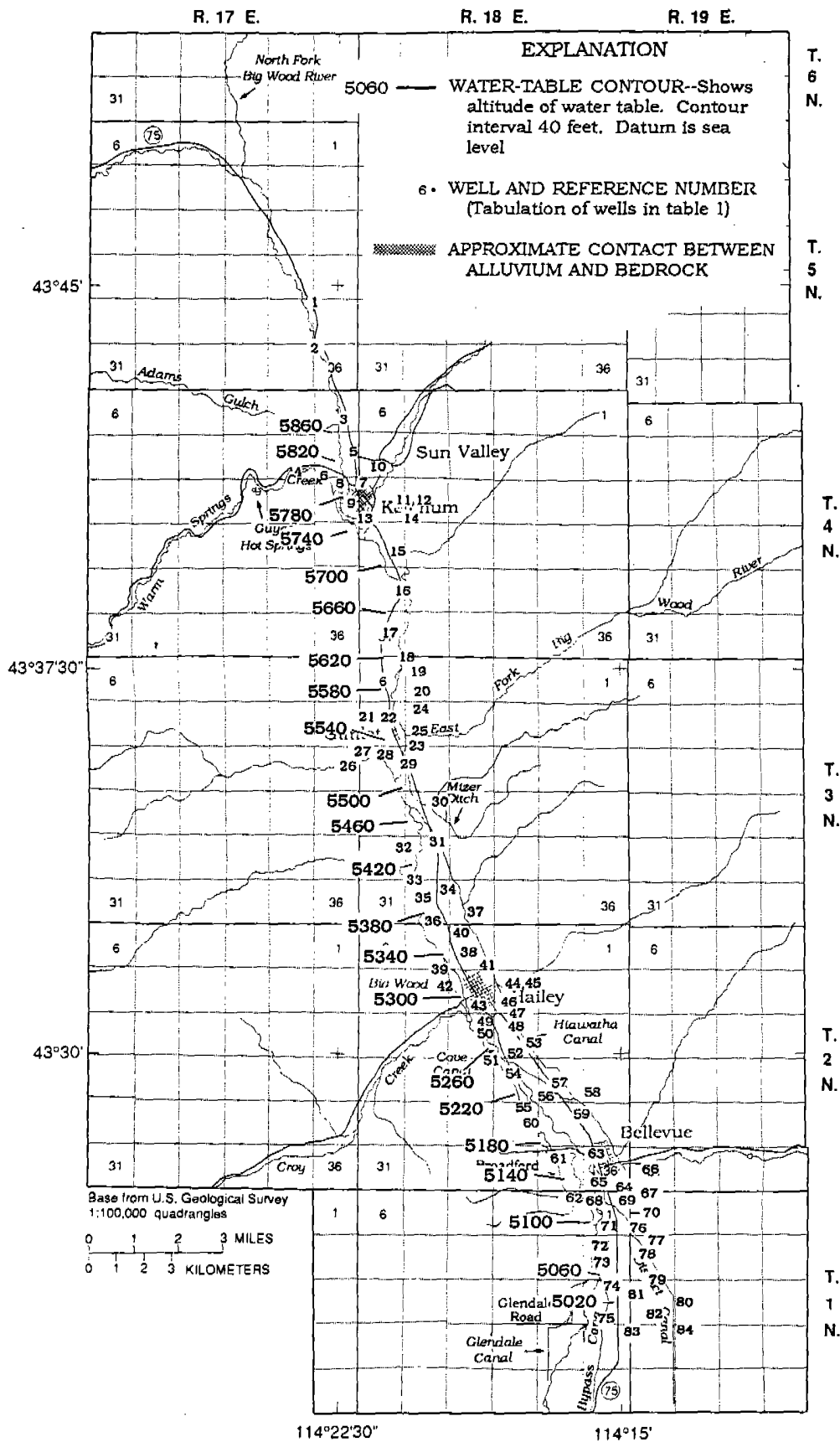
Figure 7.--Water-table contours in April 1986 and well locations
